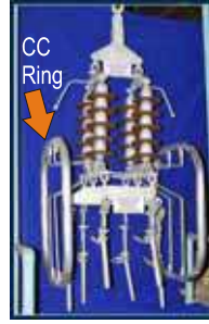
765kV Quad Tension Hardware Assembly for Hexagonal Bundle
