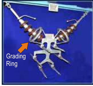
765kV V Suspension String for Hexagonal Bundle
